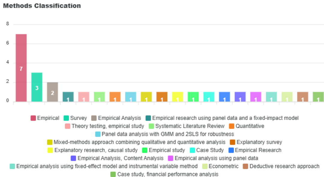
Gambar 2. Methods Classification
